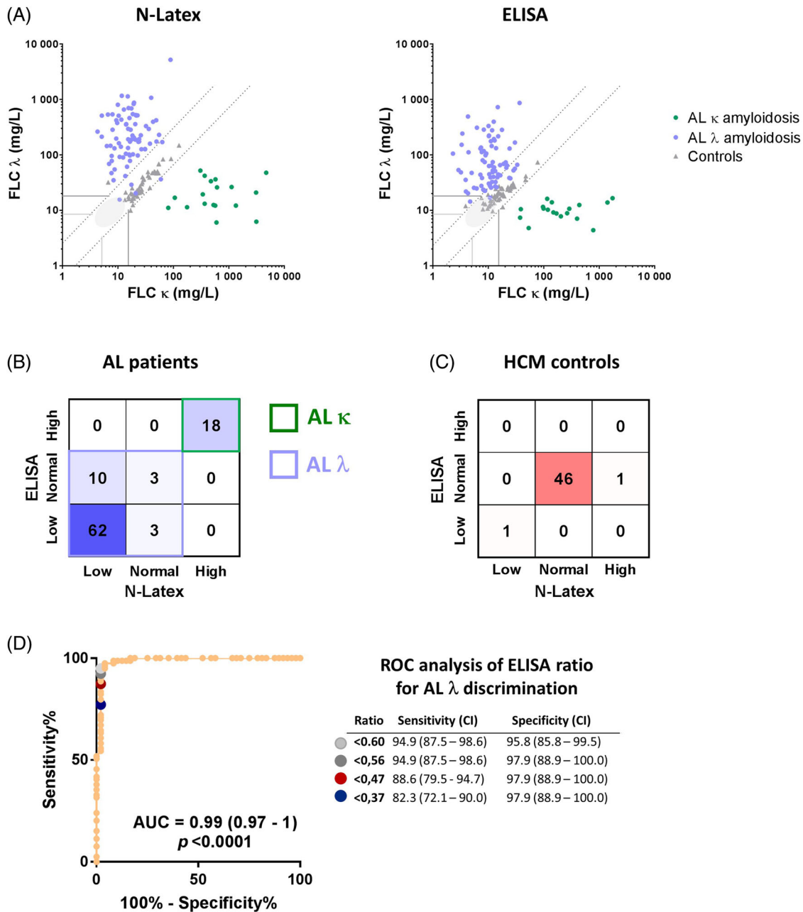
FIGURE 2 Concordance analysis and diagnostic performance. (A) Free light chain (FLC) concentrations measured by N-Latex and ELISA in patients with AL amyloidosis (green, κ AL; light blue, λ AL) and in control patients (grey triangles). The grey lines delimit lower and upper reference values for FLC concentration and κ/λ ratio; points in the light grey area have normal FLC concentrations and κ/λ ratio. (B and C) Clinical concordance analysis of the κ/λ ratio between ELISA and N-Latex within the AL cohort (B) and the control cohort (C). In B, green and blue frames delimit results for κ and λ AL amyloidosis, respectively. (D) Receiver operating characteristic (ROC) curve analysis of ELISA κ/λ ratio values from λ AL and control patients. The AUC, p value, and results for four selected cut-offs points with 95% CI are reported
